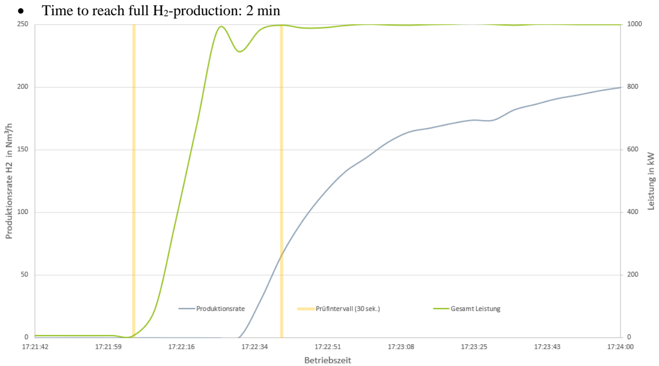
Figure 4: Time to reach full H 2 -production
